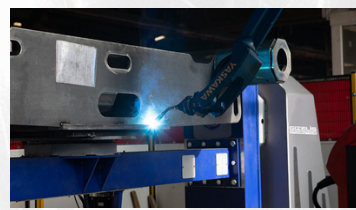
ROBOTIC WELDING OF AGRICULTURAL PARTS
